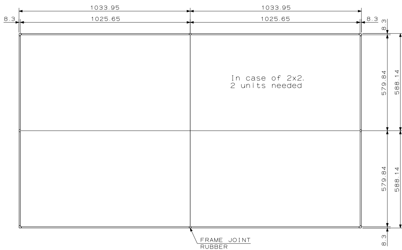
X461UN with Over-frame kit OUTLINE DRAWING
